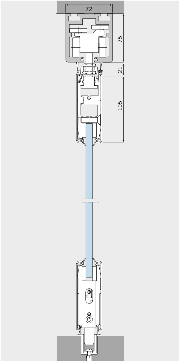
Basic Straightline element without support profile
