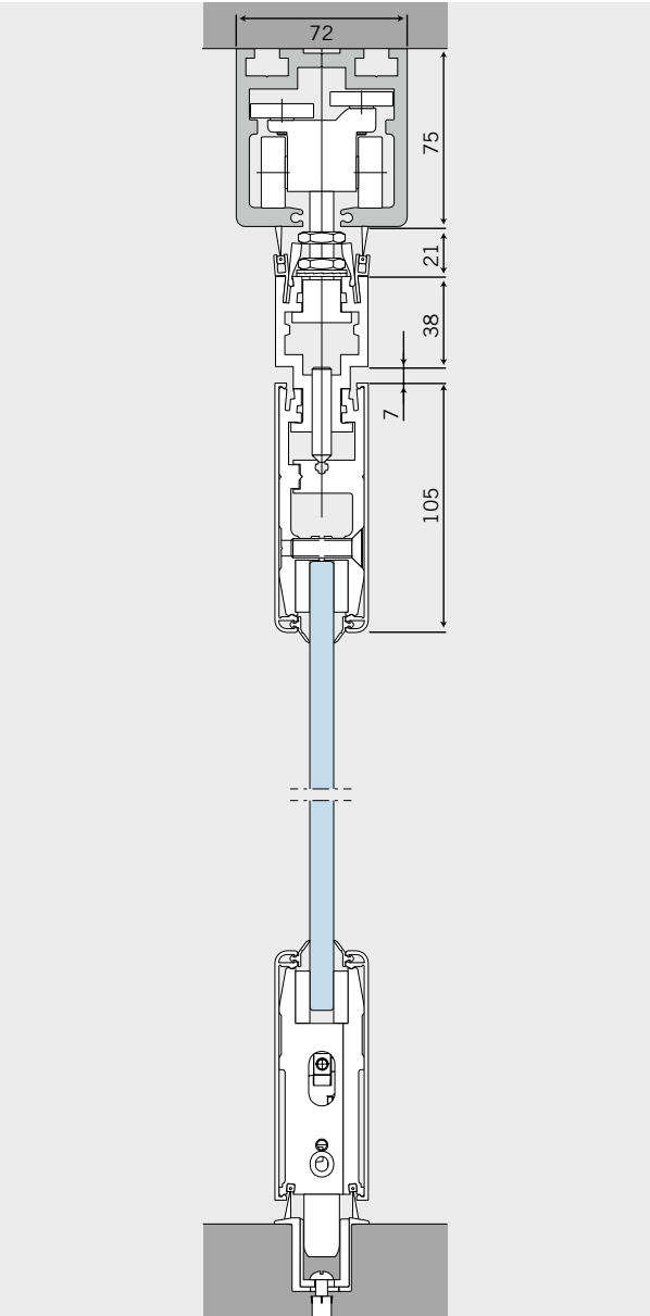
Comfort Straightline element with support profile for configurations with sliding door element
